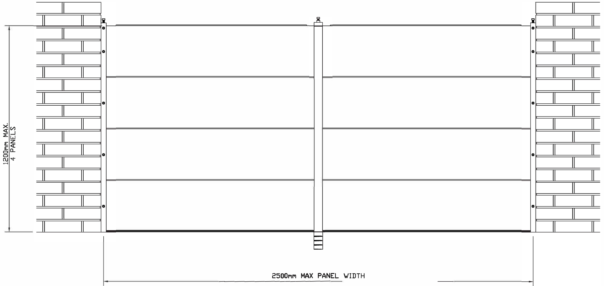
FPS BARRIER REVEAL FIX WITH COMPRESSION POST
