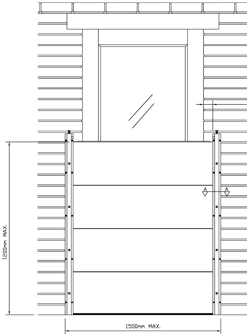
FPS BARRIER - FACE FIX
