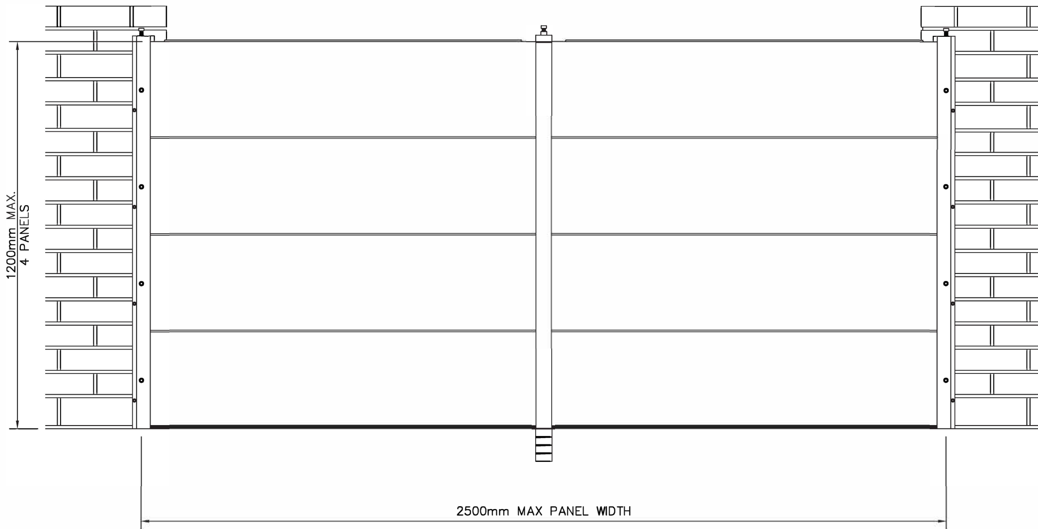
FPS BARRIER FACE FIX WITH COMPRESSION POST
